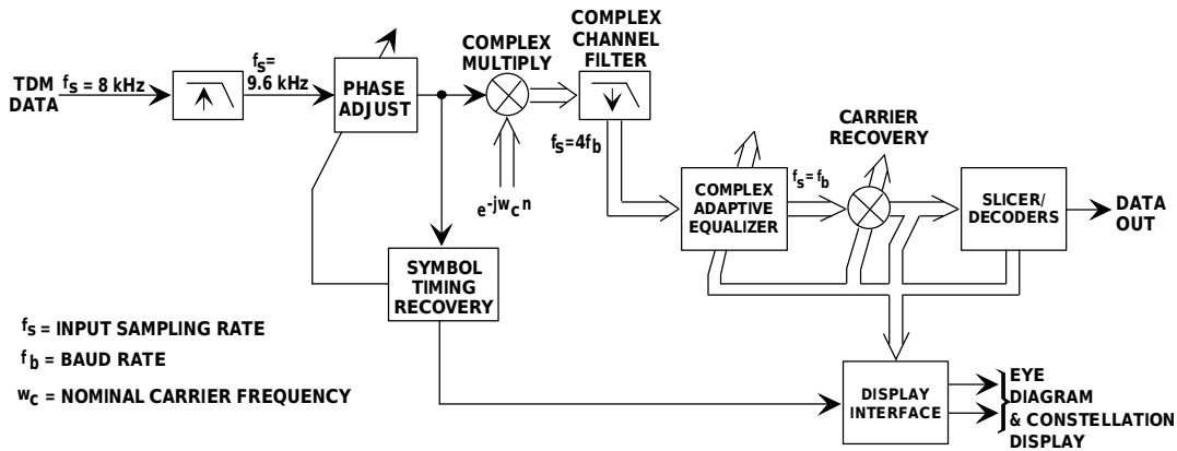
Figure 2. QAM Demodulator Algorithm
