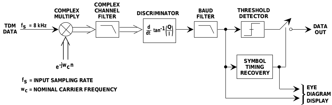
Figure 1. FSK Demodulator Algorithm
