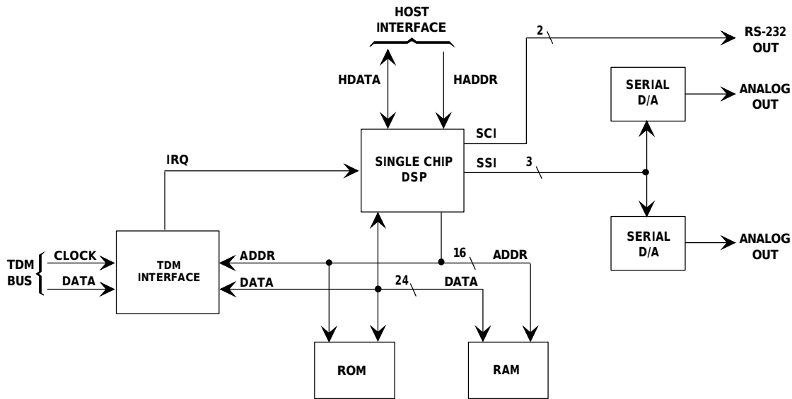
Figure 3. Block Diagram of the Option Card
